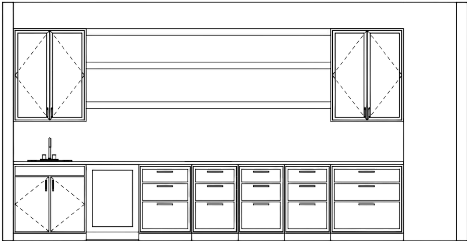
③ Elevation 1 - Bar Elevation 1/2" = 1'-0"
